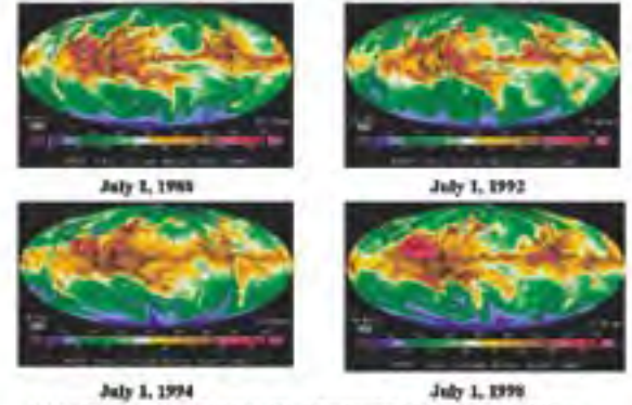
Figure 1. Examples of daily variability: Global total precipitable water from July 1 of four years. Note the large differences between days. The color scale is in units of millimeters (mm) of water. The color scale is 0 to 60 mm.
