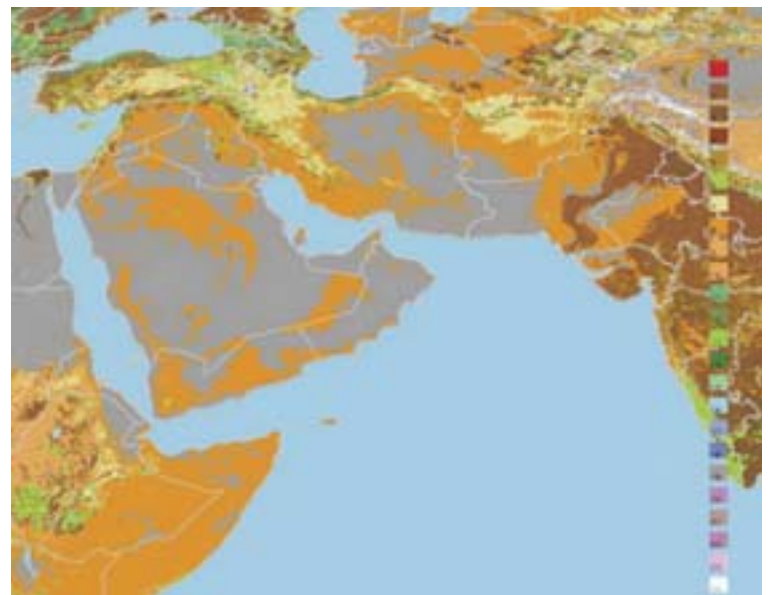
Figure 4. Data from the 1-km, global, Global Land Cover Characteristics database.
