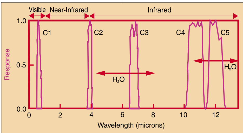
Fig.1: Spectral regions sensed by the five GOES-9 imager channels (C1-C5)
