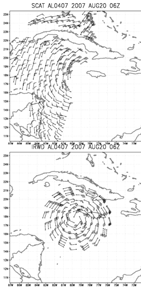
Figure 1. The input datasets to the multi-platform tropical cyclone surface wind analysis of Hurricane Dean on 20 August 2007 at 06UTC are the AMSU-based 2-D winds at 700 hPa (top left), cloud-drift and feature track winds (top right), QuickScat ocean wind vectors (bottom left) and the IR-base flight-level proxy winds (bottom right). All datasets are collected over a 12-hour period of time and moved to a storm relative position valid at 06 UTC 20 August.
